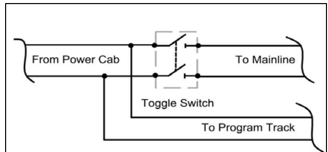
Wiring for Program Track with the Power Cab
